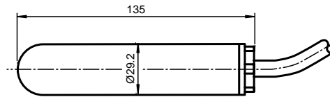
Sleeve design LFL1-CK-Z0/Z1
