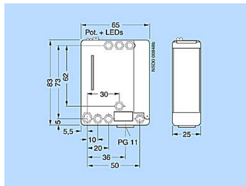
3RG72 ..-6..00-PF
