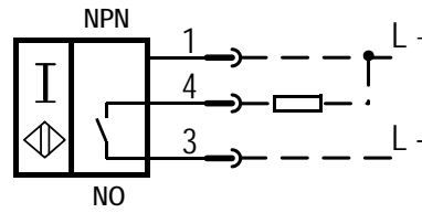
3RG4614-3GB00-PF:
