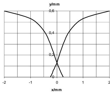
Response curve / Ansprechkennlinie
