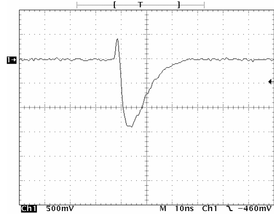
Model 50-12 Typical Output Waveform 12ns Pulse Width, 40A Output 10ns/Div horizontal scale, 20A/Div vertical
