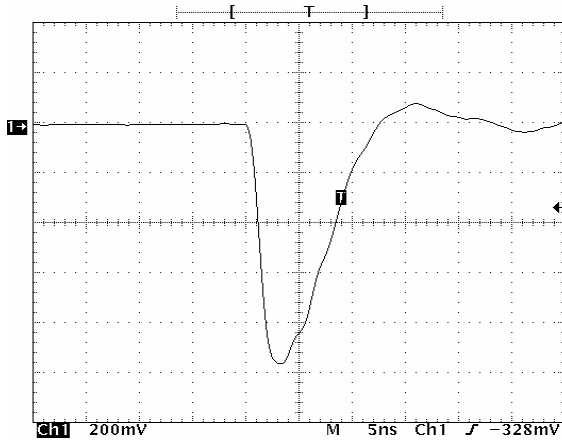
Model 40-4 Typical Output Waveform 4ns Pulse Width, 38A Output 5ns/Div horizontal scale, 8A/Div vertical
