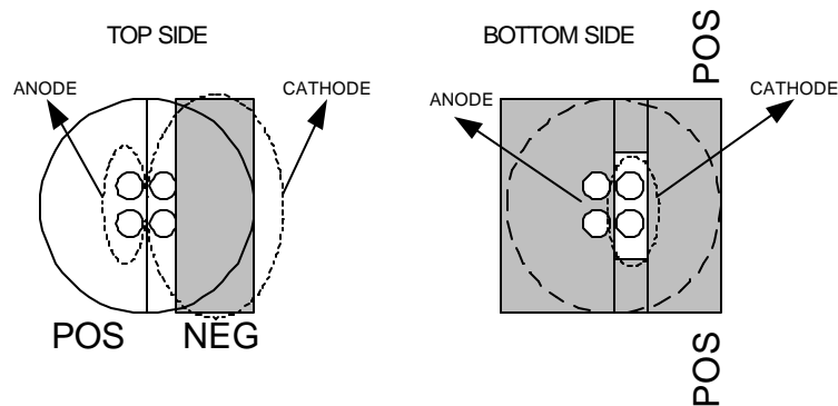
Figure 4. Detailed View of Cathode and Anode Pads on the PCB
