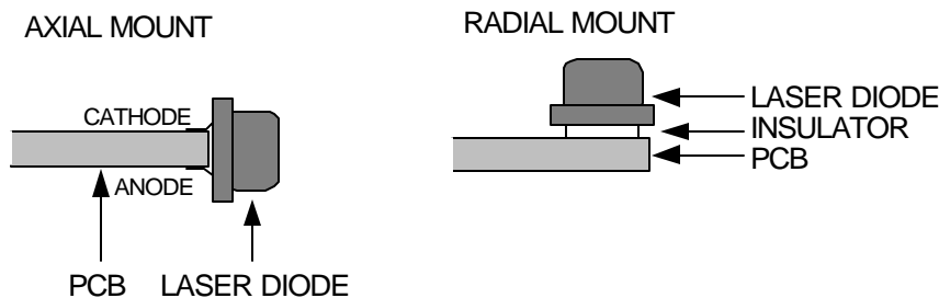
Figure 5. Axial and Radial Mounting Positions
