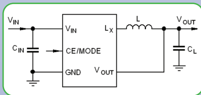
IXD3235 Schematic
