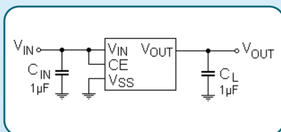
IXD1233 schematic
