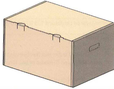
Figure 2 : New outer packaging, capacity of box-6pcs, dimensions - 390x237x255mm, inner box dimensions - 350x227x75mm
