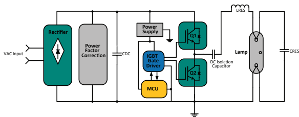
Figure 1: Electronic Lamp Ballast
