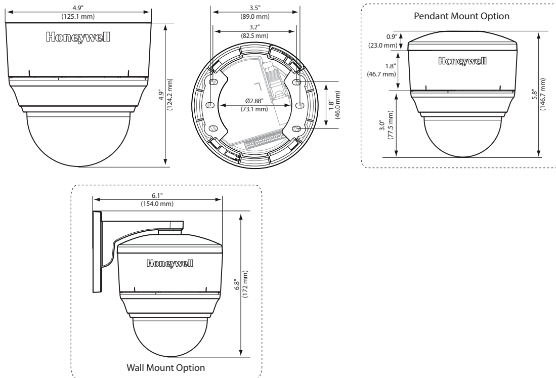
H3SVP Dimensions
