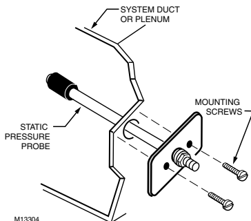
Fig. 2. Mounting static pressure probe.
