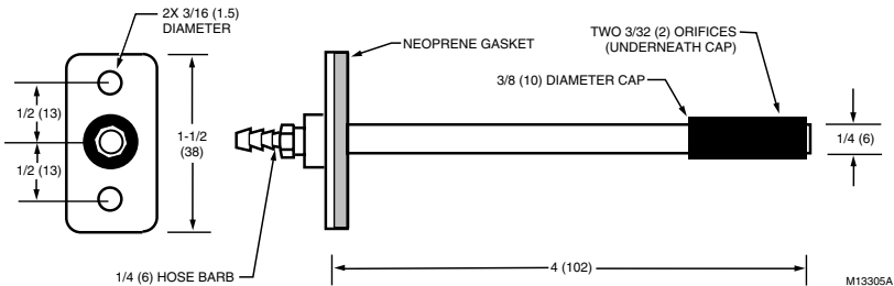
Fig. 1. 32003169-001 Static Pressure Probe dimensions in in. (mm).
