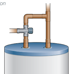
AM-1 mixing valve installation.
