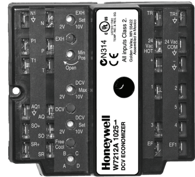
W7212, W7213 and W7214 install on flat surface or mount on M7215 motor.
