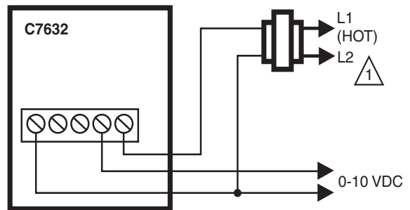
⚠ POWER SUPPLY. PROVIDE DISCONNECT MEANS AND OVERLOAD PROTECTION AS REQUIRED. M34095
