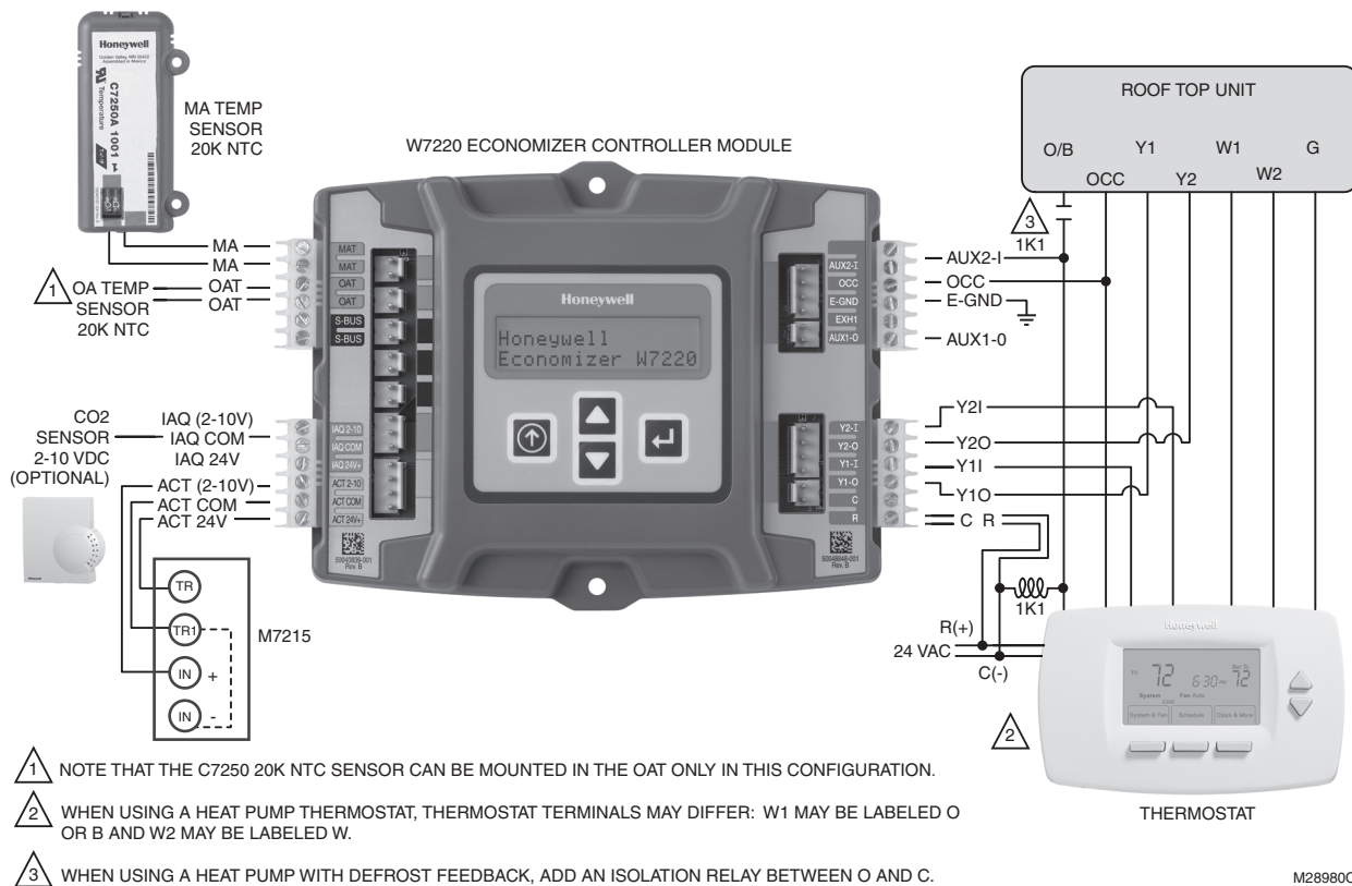
Fig. 4. Stand-alone dry bulb Economizer configuration with black motor M7215.
