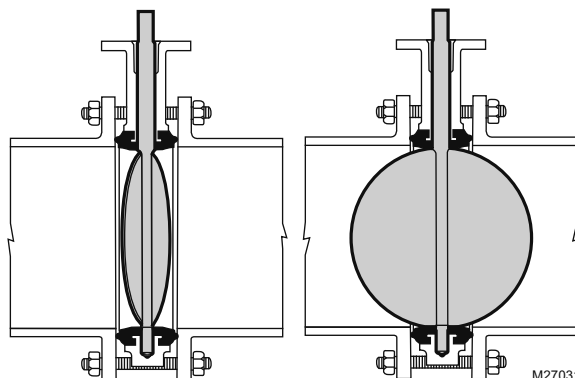
Fig. 19. Valve installation disk positions
