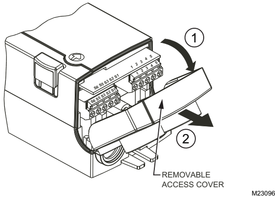
Fig. 9. Access Cover.
