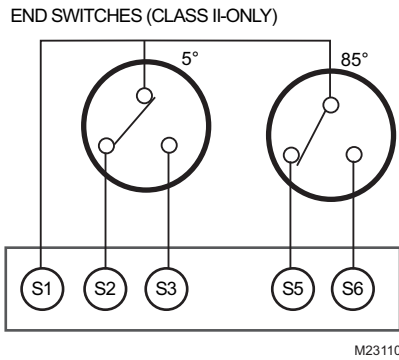
Fig. 9. End Switches.
