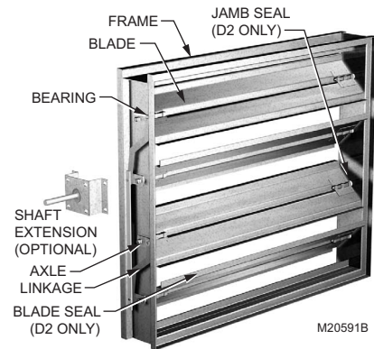
Fig. 5. Damper components.
