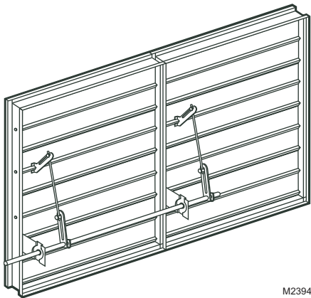
Fig. 4. Multiple section damper.
