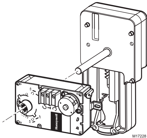
Fig. 5. Installing 35 or 70 lb-in. actuator.
