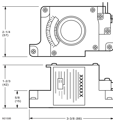
Fig. 1. Dimension drawing in in. (mm).
