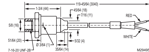
Fig. 2. MLH01KPSCDJ1241/MLH500PSCDJ1240 dimensions in in. (mm).
