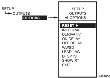
Fig. 31. Configuration - Sorties - Menu Options.
