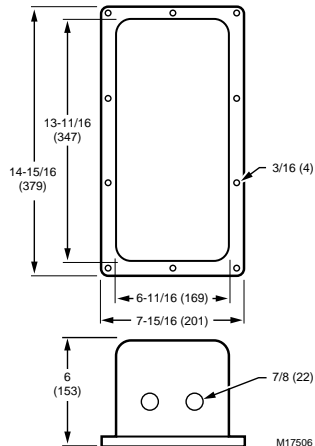
Fig. 1. Dimensions of 32003036-001.
