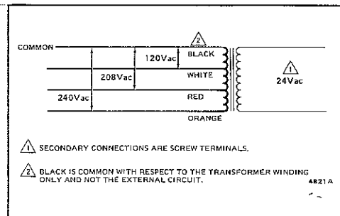
Fig. 7—Transformer schematic.
