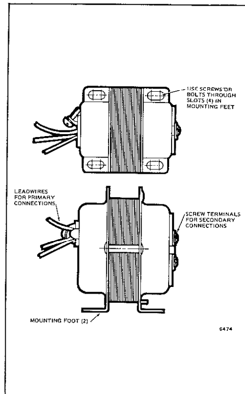
Fig. 1—Foot mounting.
