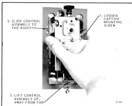
Fig. 2—Mounting the control on the backplate.
