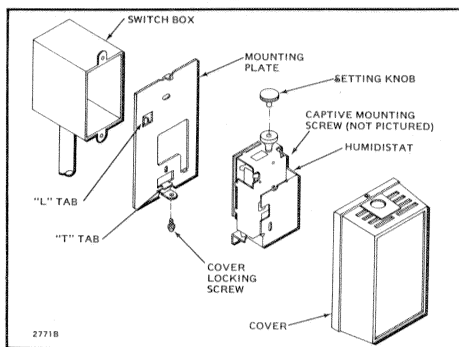
Fig. 1—H600A backplate mounting.
