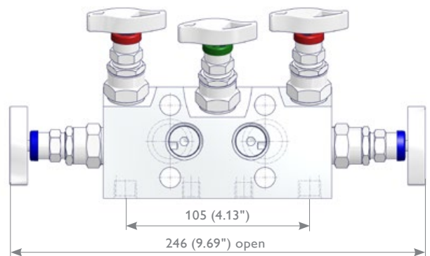
Illustrated type with IEC 61518-B connection
