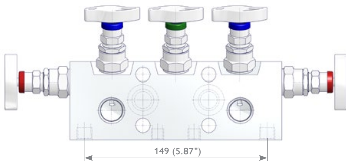
Illustrated type with IEC 61518-A connection
