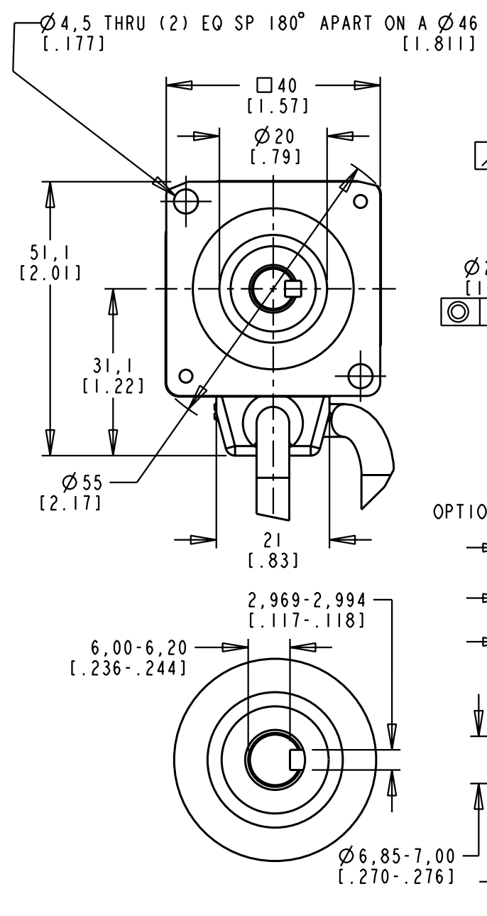
SHAFT DETAIL (NO SCALE)
