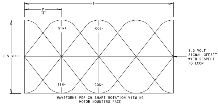
SIN+, SIN-, COS+, COS- ENCODER OUTPUT WAVEFORMS
