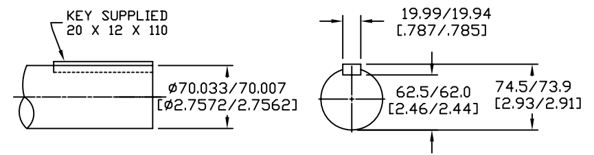
DRIVE END SHAFT DETAIL SPEC (9)
