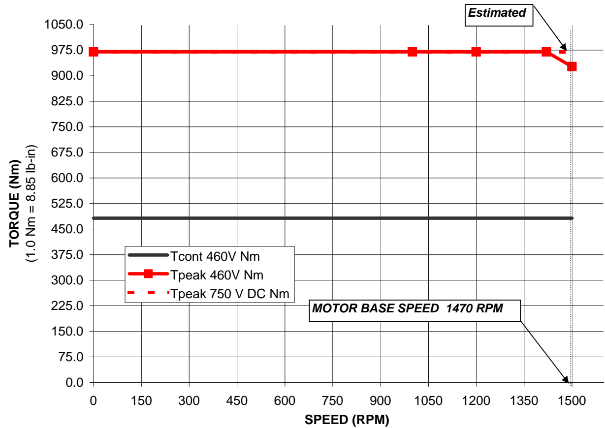
HPA-B2010C-SC44AA Performance with 2099-BM11 at 460 VAC and 750 V DC Drive Input, 40C Motor Ambient
