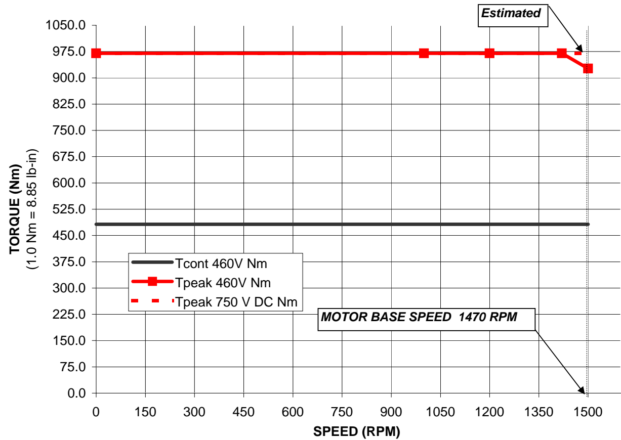
HPA-B2010C-SB44AA Performance with 2099-BM11 at 460 VAC and 750 V DC Drive Input, 40C Motor Ambient
