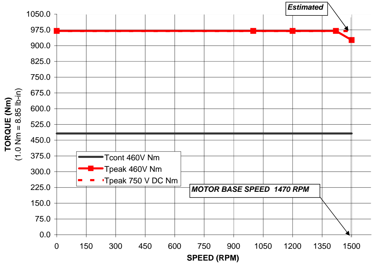
HPA-B2010C-SA42AA Performance with 2099-BM11 at 460 VAC and 750 V DC Drive Input, 40C Motor Ambient
