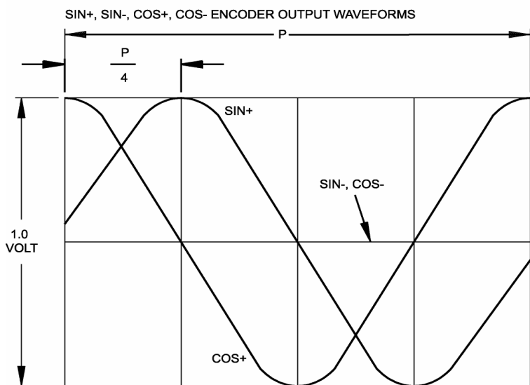
WAVEFORMS PER CW SHAFT ROTATION VIEWING MOTOR MOUNTNG FACE
