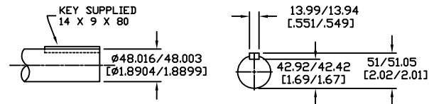
DRIVE END SHAFT DETAIL SPEC (9)
