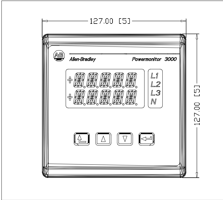
1404-DM Powermonitor 3000 Display Module
