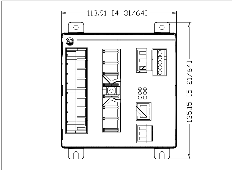
1404-M Powermonitor 3000 Master Module
