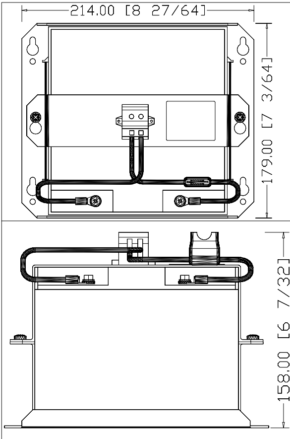
1606-XLSBATASSY2 Battery assembly with bracket, for use with DC UPS, 26Ah, 12V
