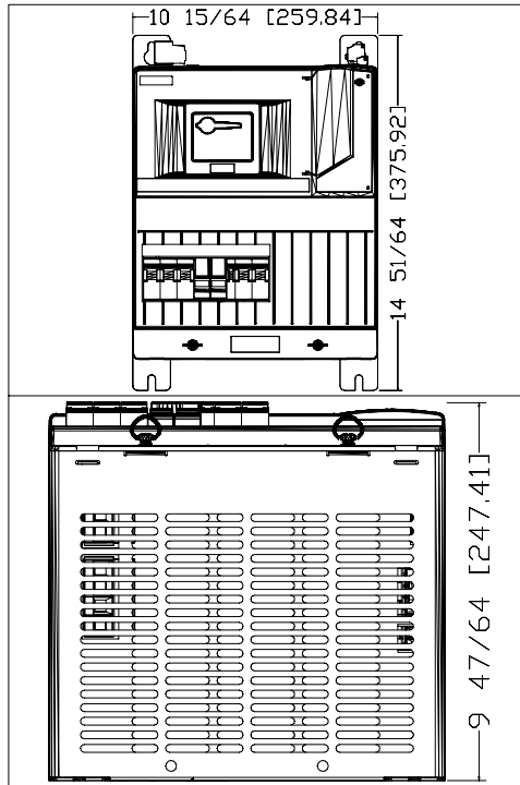
2094-BL75S Module, Line Interface 75A, 460VAC
