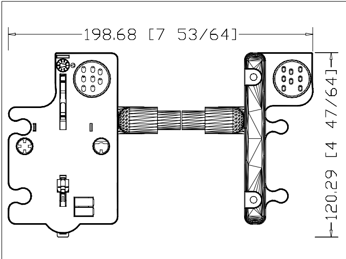
1738-EXT1 ArmorPoint 1 Meter Bus Extension Base
