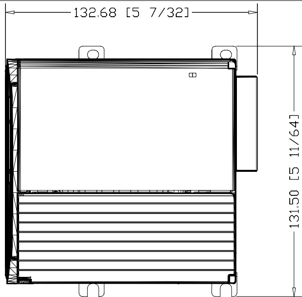
1768-PA3 CompactLogix AC Power Supply
