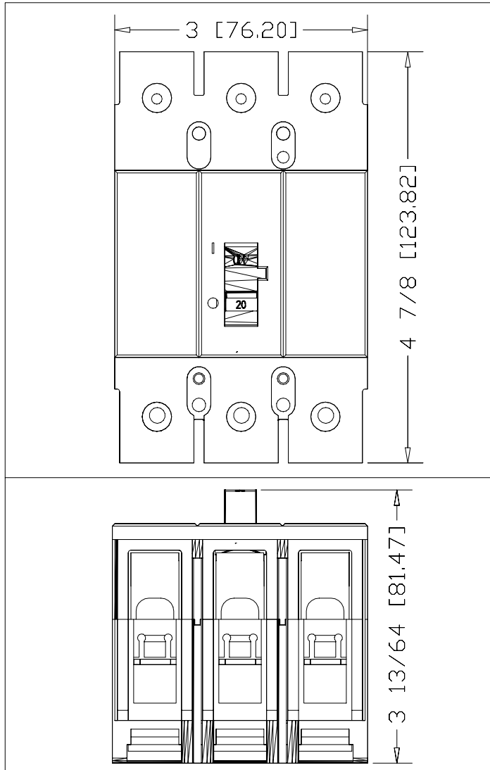
140U-G* Molded Case Circuit Breakers, 100 Amp, 3-Pole, G-Frame
