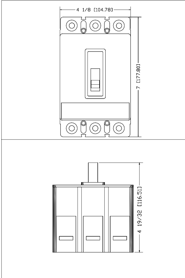
140U-J* MOLDED CASE CIRCUIT BREAKERS, 250 AMP J-FRAME
