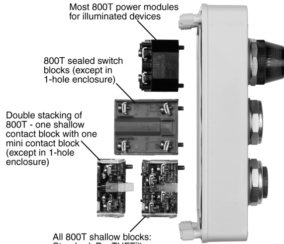
Bul. 800H – 30.5 mm Push Button Enclosure
