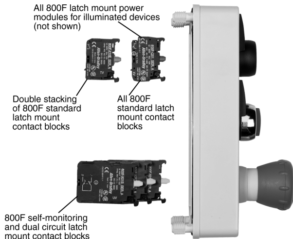
Bul. 598 – 22.5 mm Push Button Enclosure
