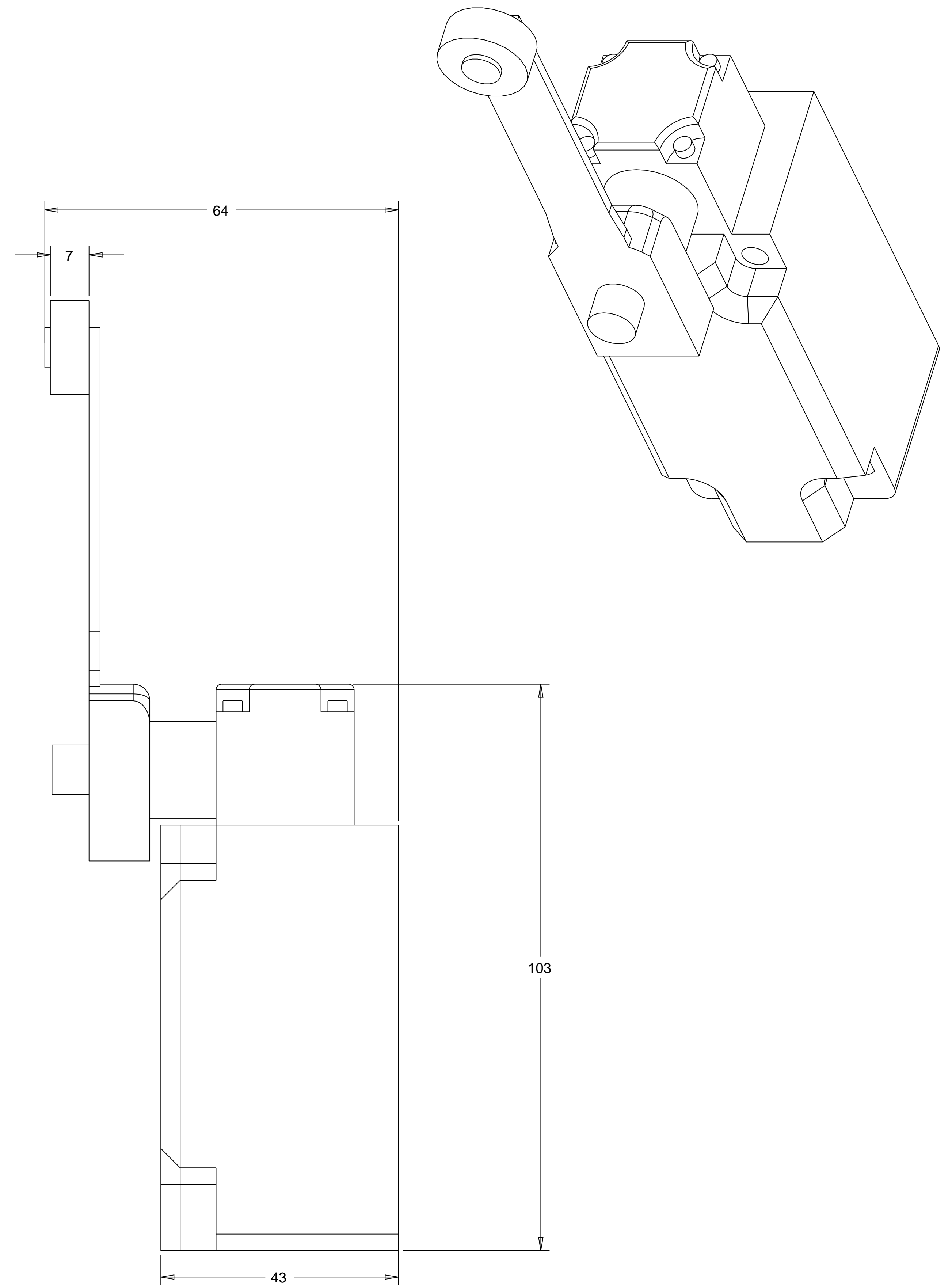
440P_ADJUSTABLE_LEVER_SENSOR
