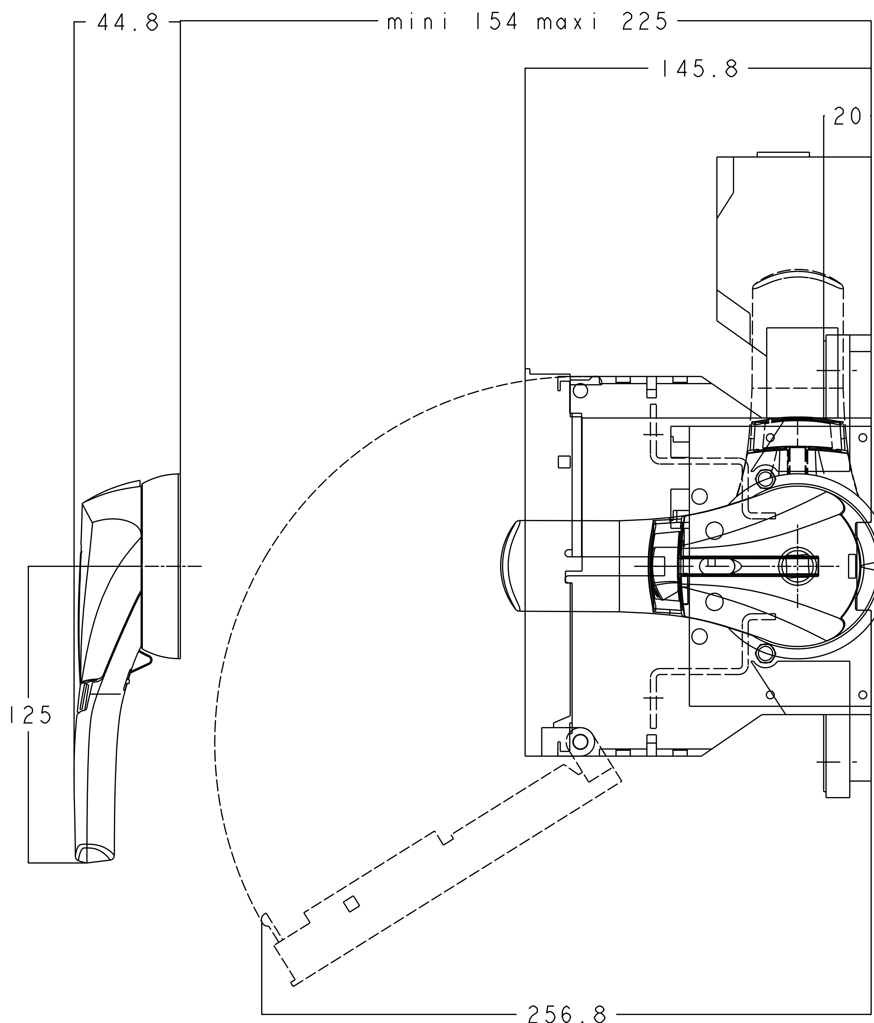
BOX DRILLING SIDE
