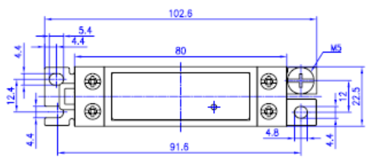
WITH M5 EARTH TERMINATION BOLT
